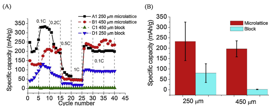
Fig. 5. (A) Specific capacity of the microlattice and block electrodes as a function of number of cycles at different C-rates. (B) Comparison of the average specific capacity of microlattice and block structure thicknesses of 250 μm and 450 μm.
