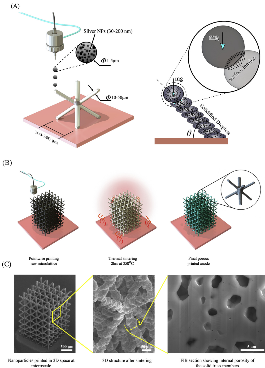
Fig. 2. (A) Schematic of the fabrication of 3D micro-architected battery electrodes by assembling nanoparticles in 3D space at microscale using the aerosol jet printing process. Heat removes the binders and sinters the nanoparticles to form the 3D microlattice with hierarchical porosity. (B) Schematic of the formation of 3D microlattice. (C) Representative SEM images of the 3D microlattice fabricated by the process described in (A) and (B). The FIB image shows a representative section of the truss member of the microlattice. Porosity at a length scale of 100 microns or more is seen from printing; while porosity at a length scale of about a micron is seen within the truss members.
